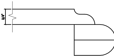
OGEE WITH STEPPED LAMINATED BULLNOSE
