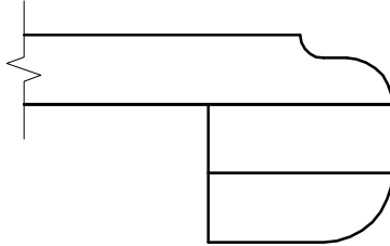
TRIPLE LAMINATION OGEE BULLNOSE
